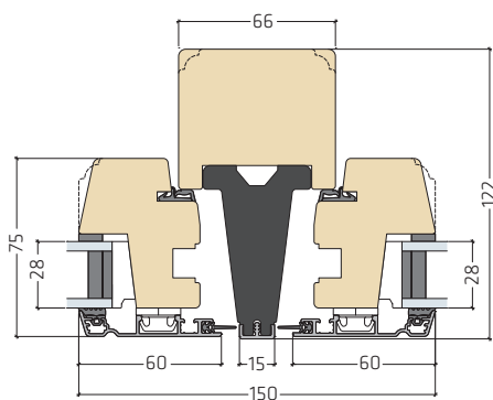
FRAic01-50L28 | Lodret post
