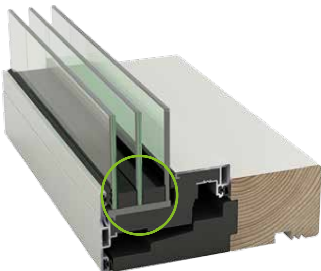
Warm edge Reduces the thermal bridge
